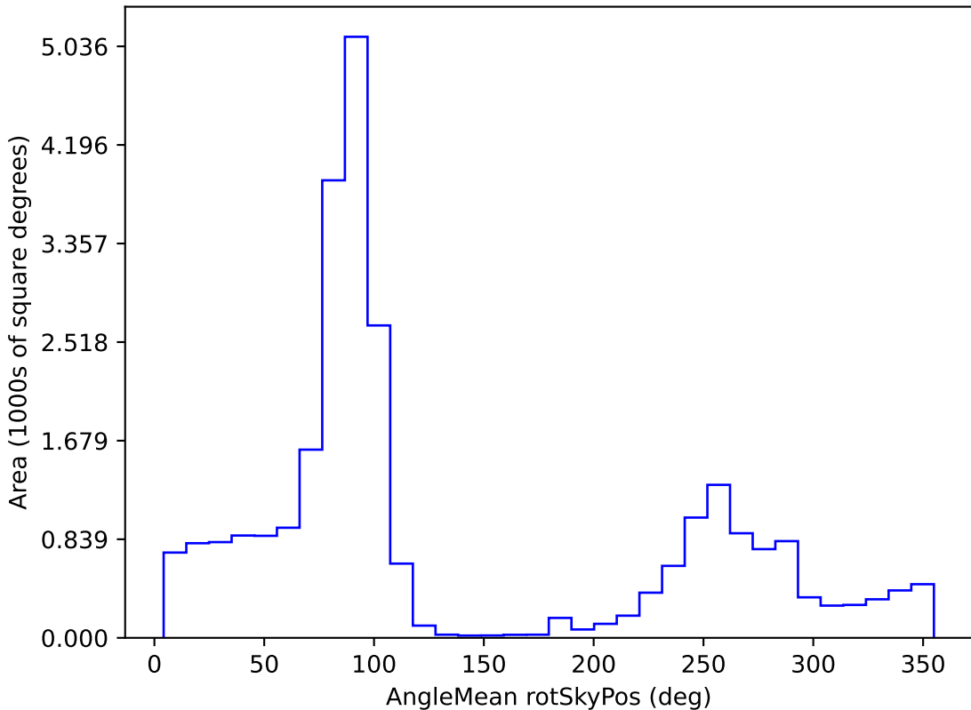
weather_cloudso0v3.5_10yrs All sky r band: AngleMean rotSkyPos
