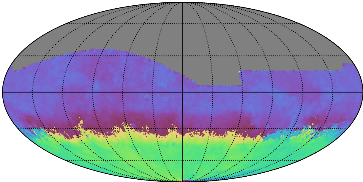
weather_cloudso0v3.5_10yrs All sky g band: AngleMean rotSkyPos
