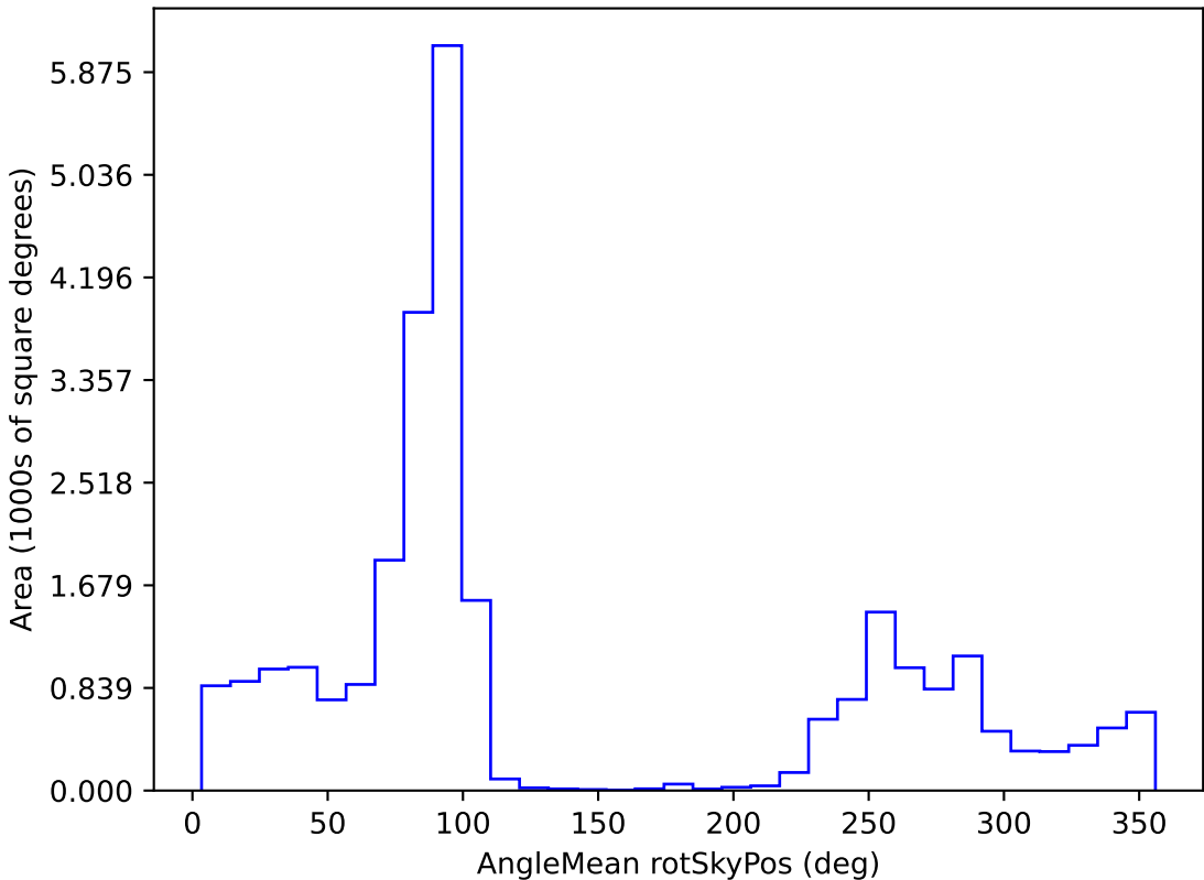
weather_cloudso0v3.5_10yrs All sky all bands: AngleMean rotSkyPos
