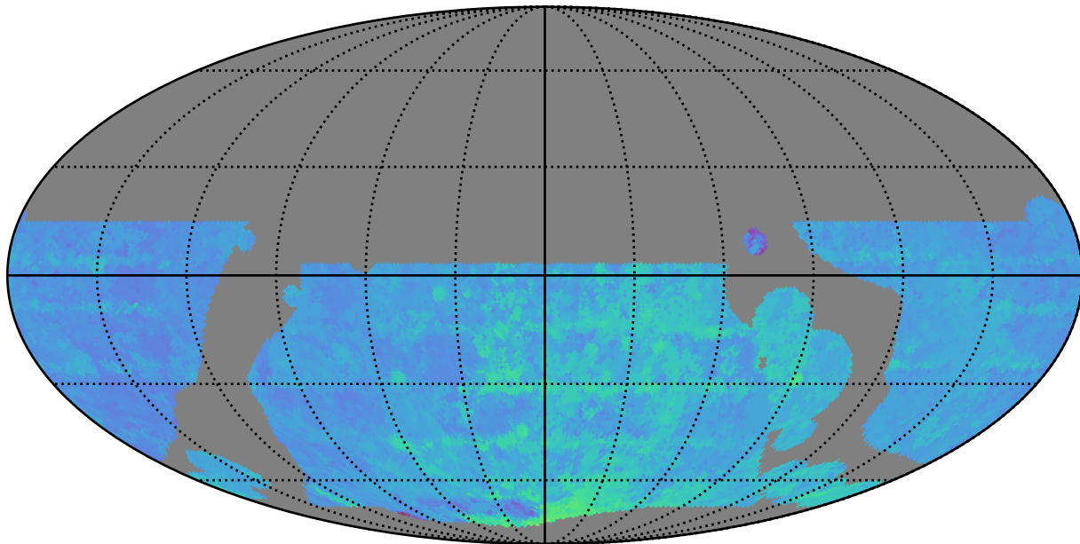
weather_cloudso0v3.5_10yrs WFD z band: 80thPercentile Season Length
