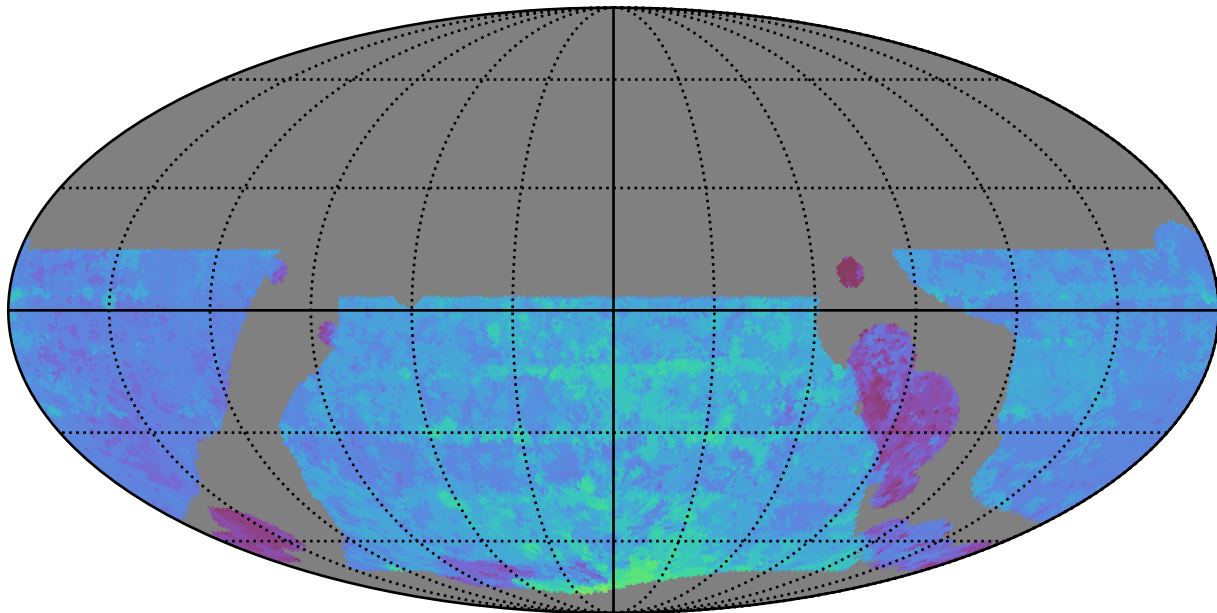
weather_cloudso0v3.5_10yrs WFD y band: 80thPercentile Season Length
