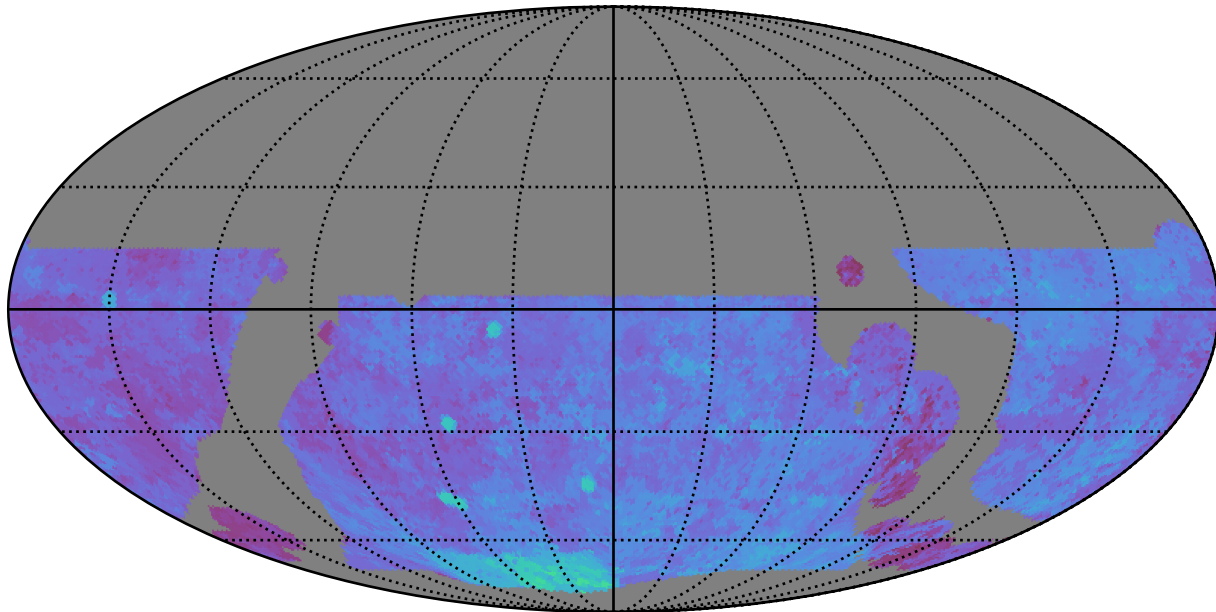
weather_cloudso0v3.5_10yrs WFD u band: 80thPercentile Season Length
