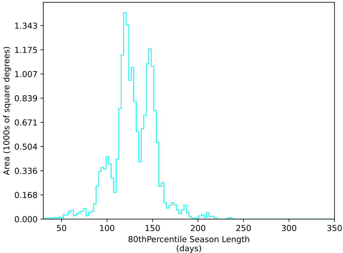
weather_cloudso0v3.5_10yrs WFD u band: 80thPercentile Season Length
