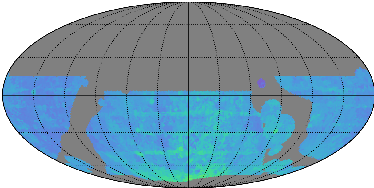
weather_cloudso0v3.5_10yrs WFD r band: 80thPercentile Season Length
