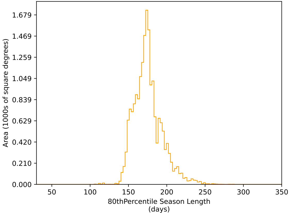
weather_cloudso0v3.5_10yrs WFD r band: 80thPercentile Season Length
