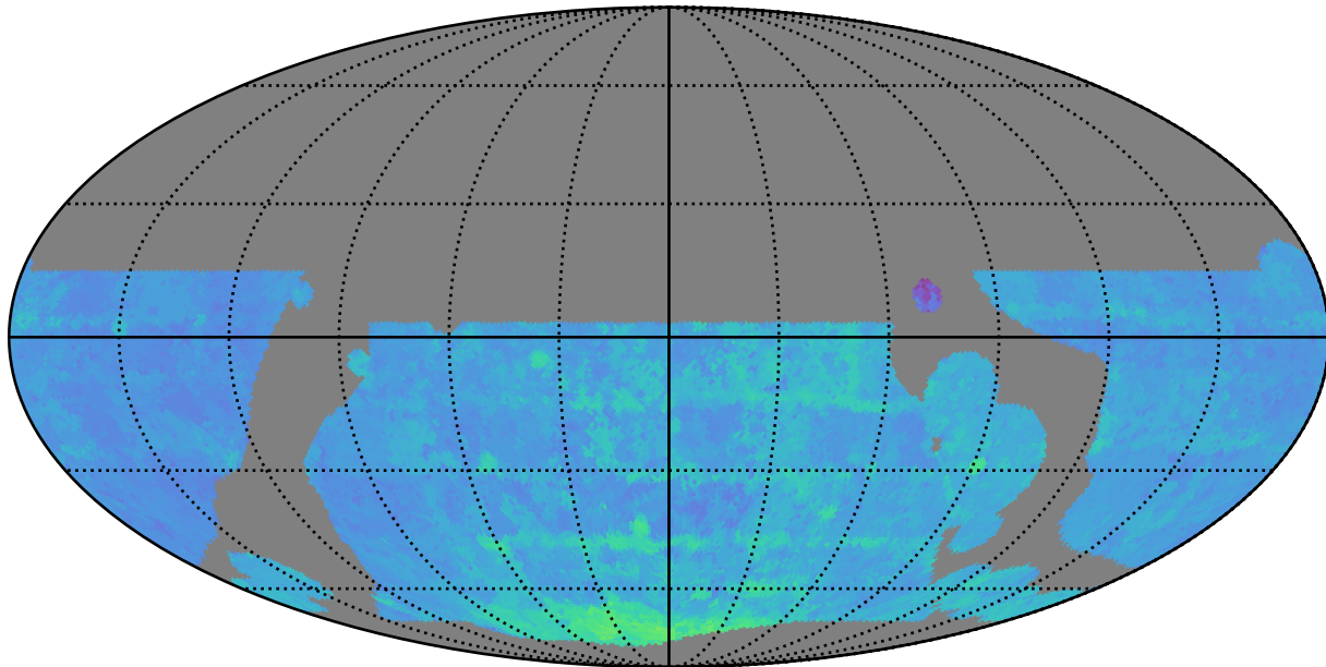
weather_cloudso0v3.5_10yrs WFD i band: 80thPercentile Season Length
