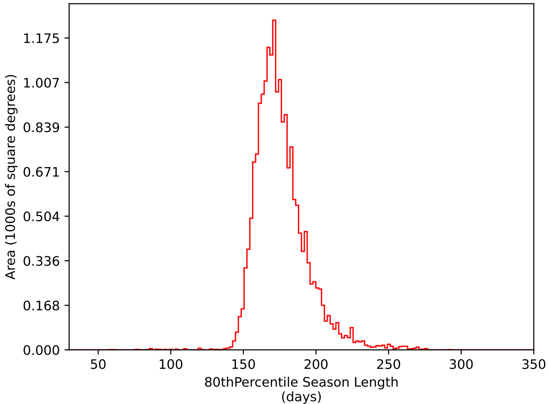
weather_cloudso0v3.5_10yrs WFD i band: 80thPercentile Season Length
