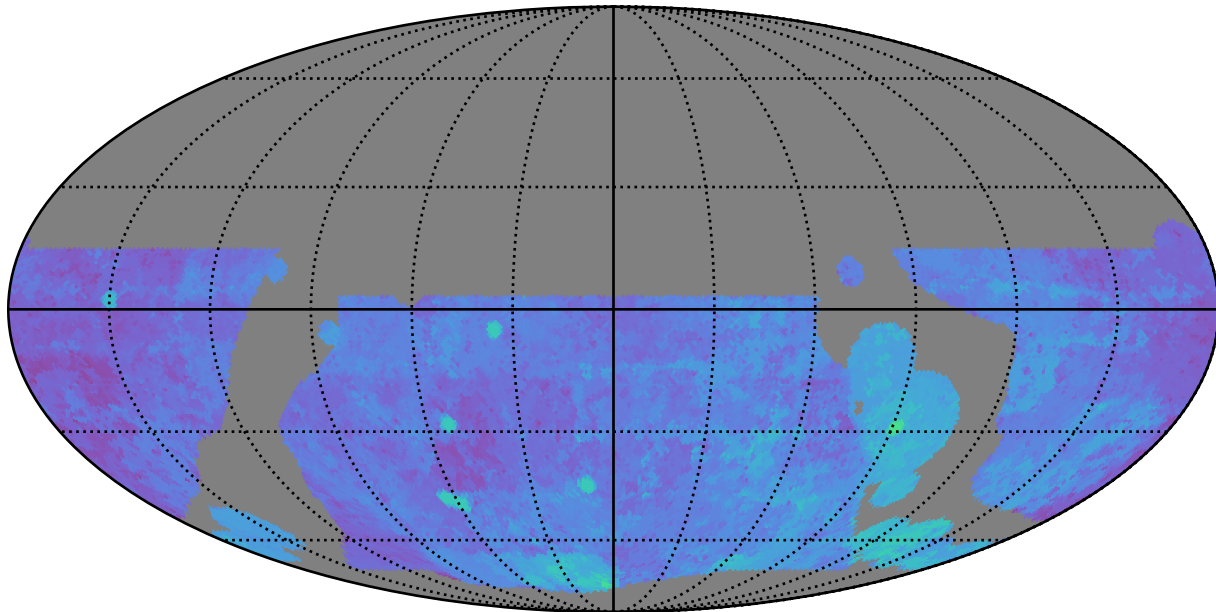
weather_cloudso0v3.5_10yrs WFD g band: 80thPercentile Season Length
