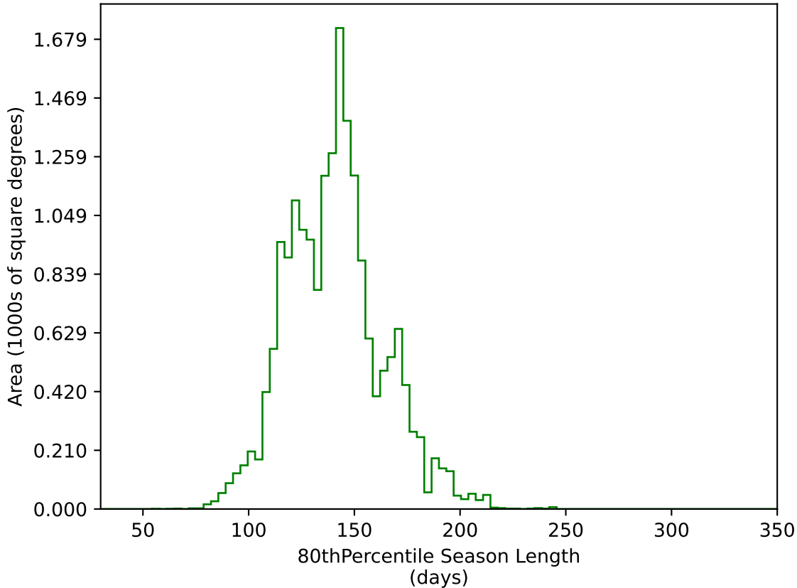
weather_cloudso0v3.5_10yrs WFD g band: 80thPercentile Season Length
