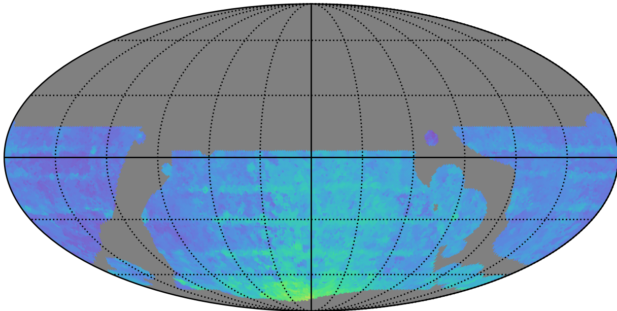
weather_cloudso0v3.5_10yrs WFD all bands: 80thPercentile Season Length
