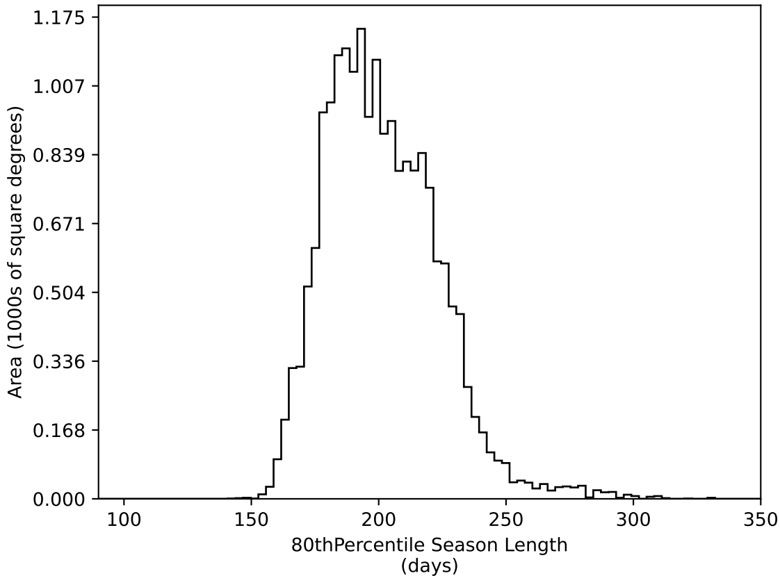
weather_cloudso0v3.5_10yrs WFD all bands: 80thPercentile Season Length
