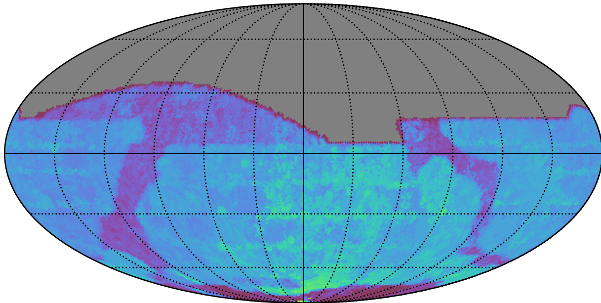
weather_cloudso0v3.5_10yrs All sky z band: 80thPercentile Season Length
