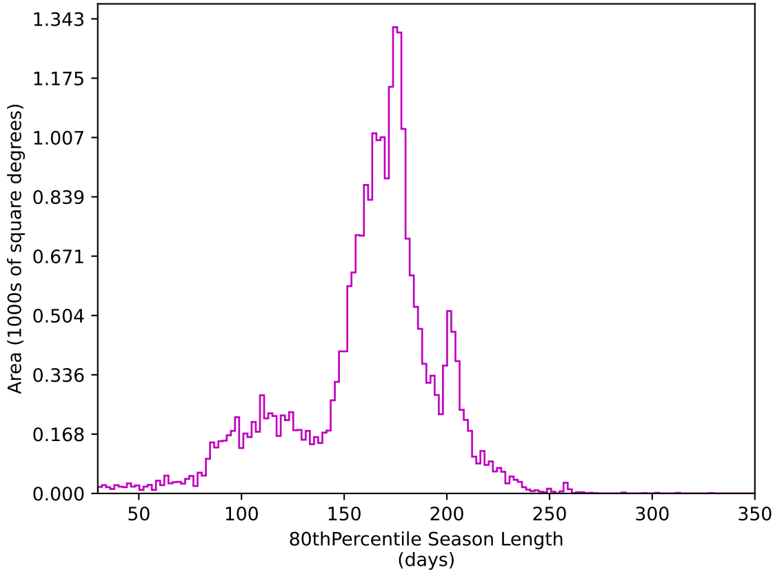
weather_cloudso0v3.5_10yrs All sky z band: 80thPercentile Season Length
