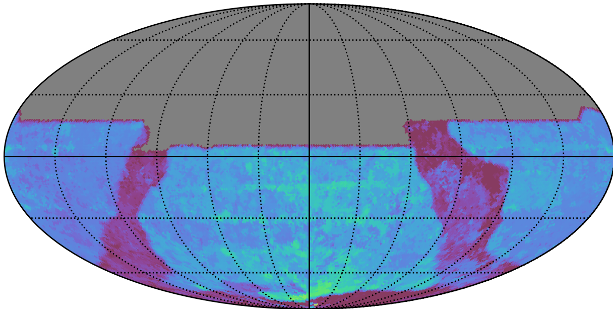
weather_cloudso0v3.5_10yrs All sky y band: 80thPercentile Season Length
