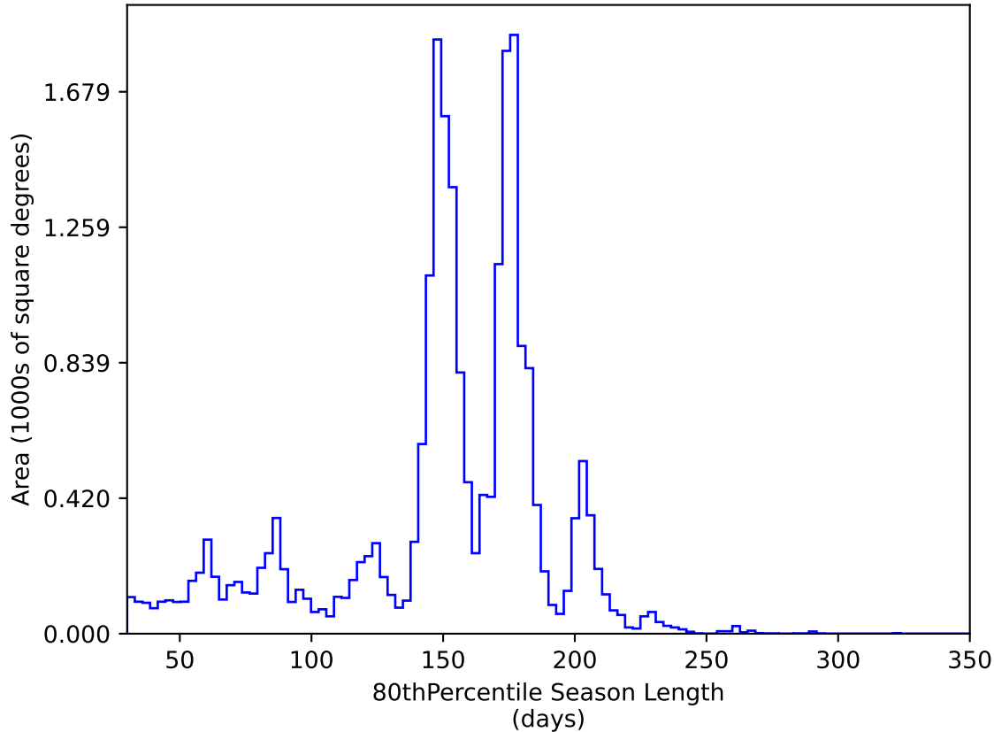
weather_cloudso0v3.5_10yrs All sky y band: 80thPercentile Season Length
