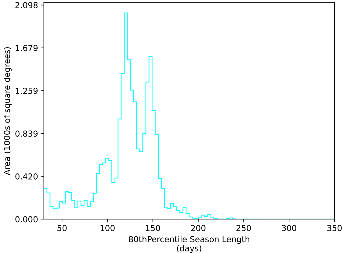
weather_cloudso0v3.5_10yrs All sky u band: 80thPercentile Season Length
