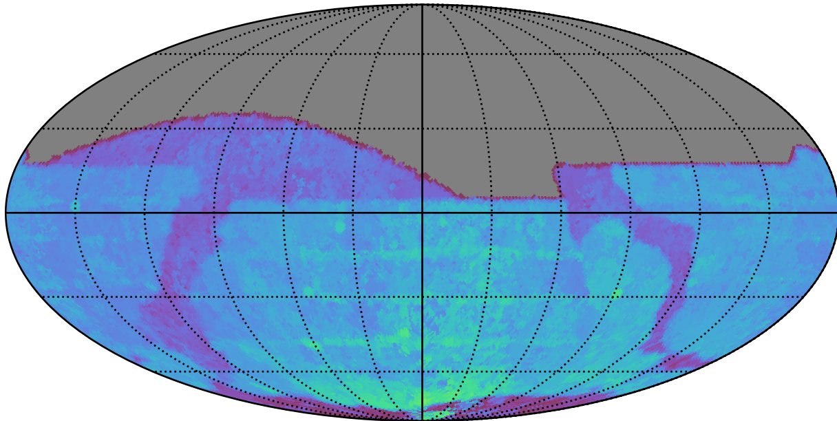
weather_cloudso0v3.5_10yrs All sky r band: 80thPercentile Season Length
