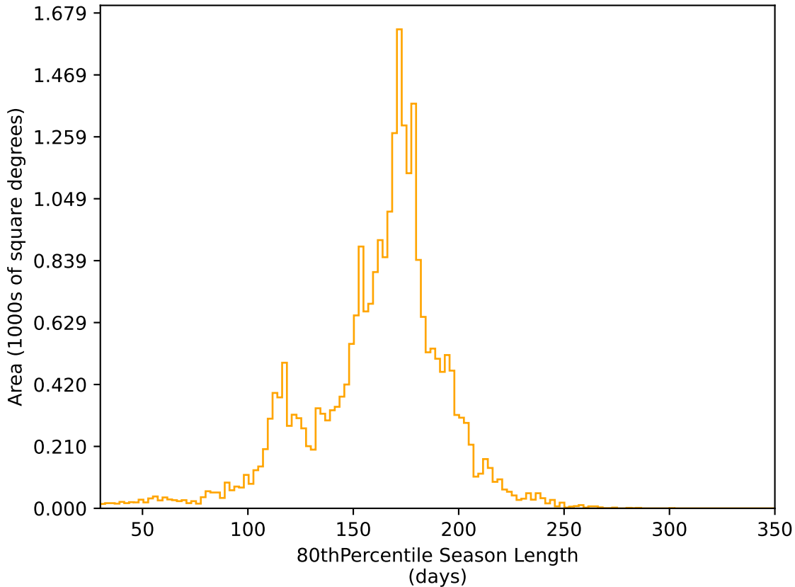
weather_cloudso0v3.5_10yrs All sky r band: 80thPercentile Season Length
