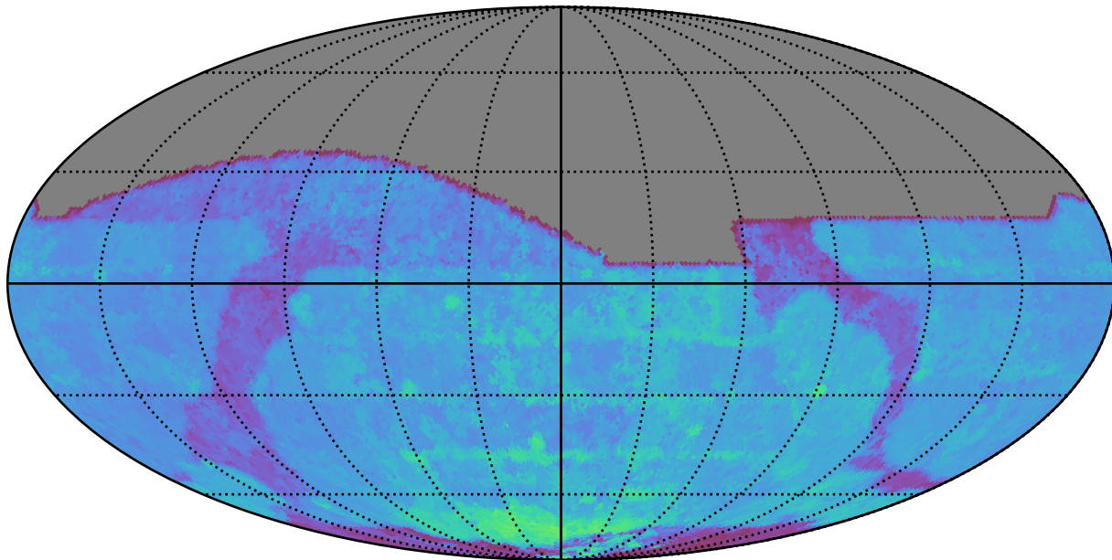
weather_cloudso0v3.5_10yrs All sky i band: 80thPercentile Season Length
