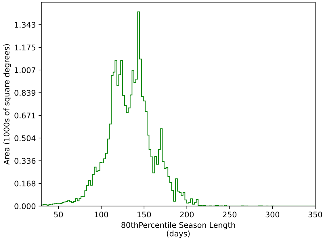
weather_cloudso0v3.5_10yrs All sky g band: 80thPercentile Season Length
