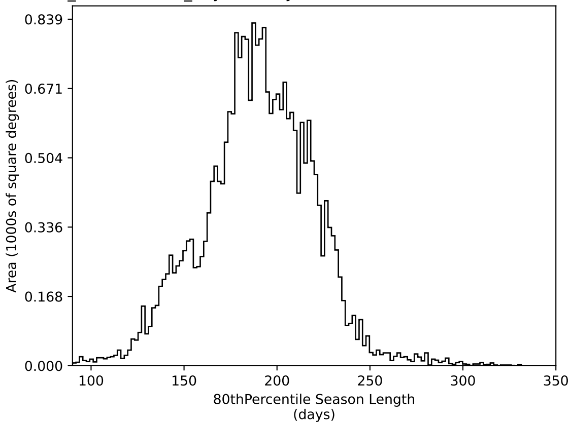
weather_cloudso0v3.5_10yrs All sky all bands: 80thPercentile Season Length
