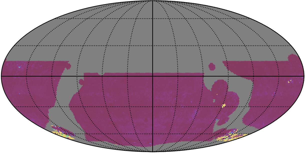
weather_cloudso0v3.5_10yrs WFD zy bands: 75th Percentile Intranight Timespan
