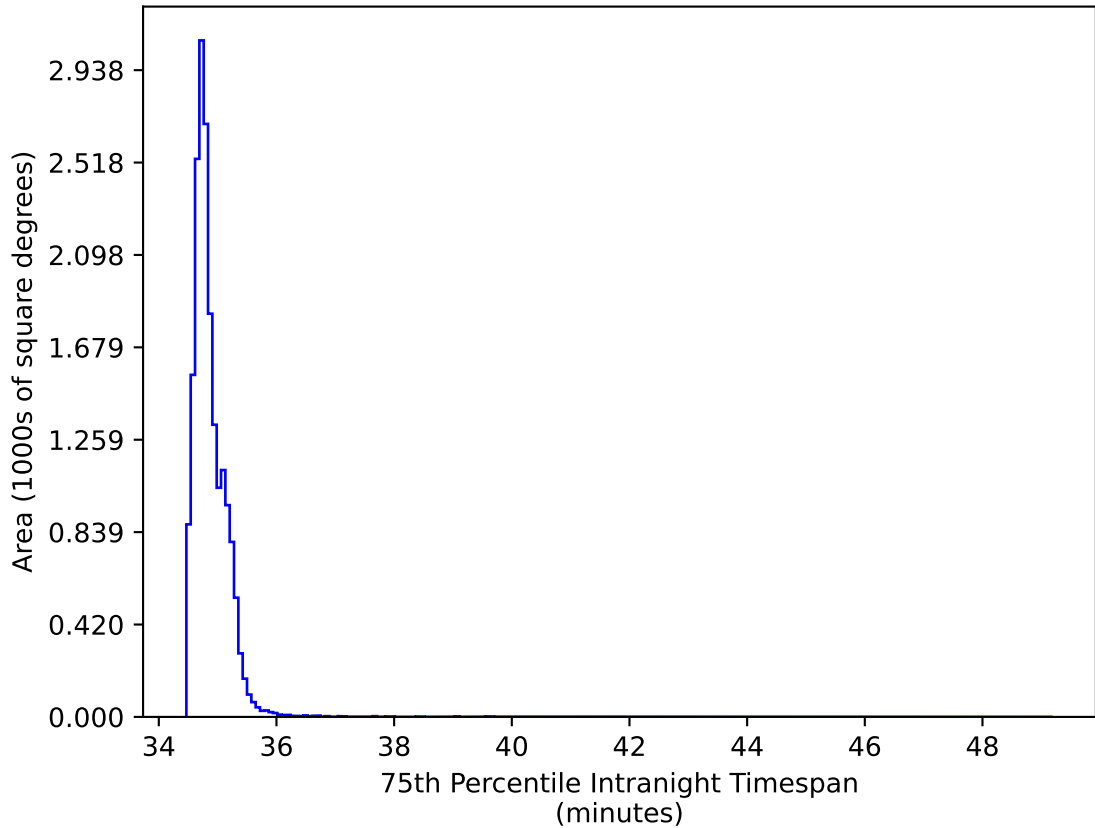
weather_cloudso0v3.5_10yrs WFD zy bands: 75th Percentile Intranight Timespan
