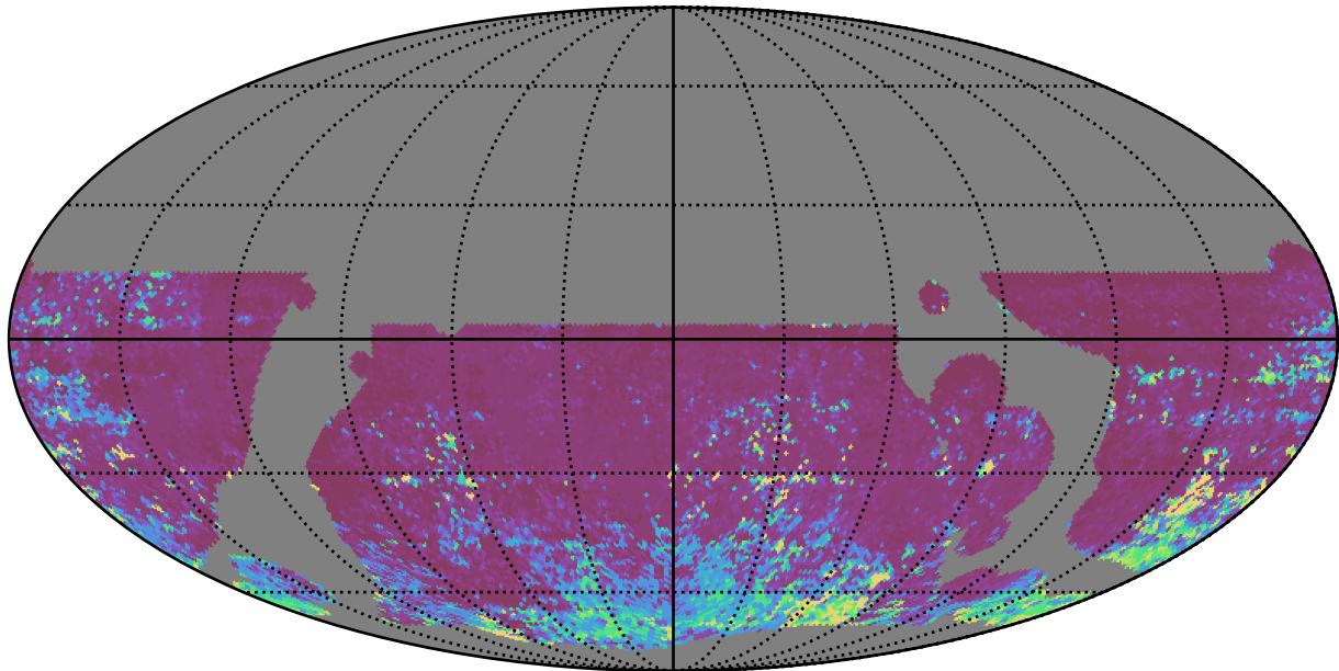
weather_cloudso0v3.5_10yrs WFD z band: 75th Percentile Intranight Timespan
