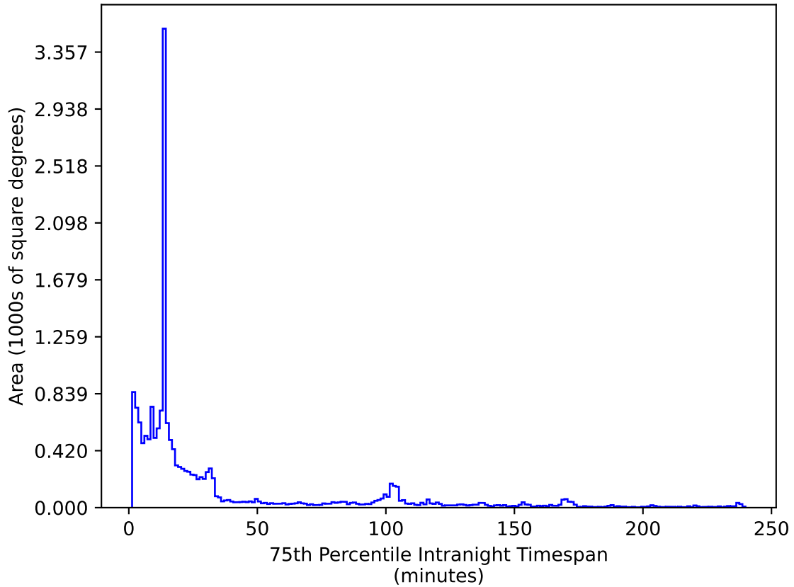
weather_cloudso0v3.5_10yrs WFD z band: 75th Percentile Intranight Timespan
