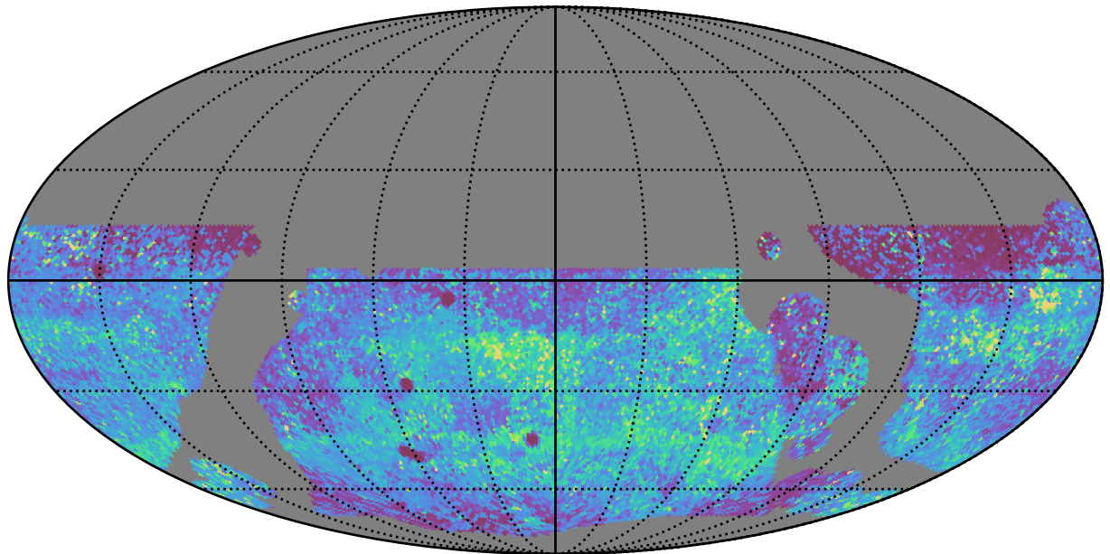
weather_cloudso0v3.5_10yrs WFD y band: 75th Percentile Intranight Timespan
