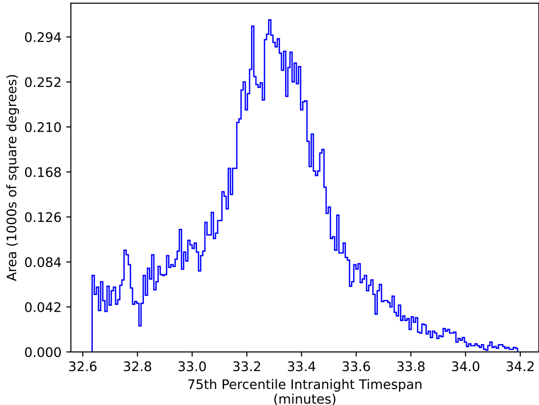
weather_cloudso0v3.5_10yrs WFD y band: 75th Percentile Intranight Timespan
