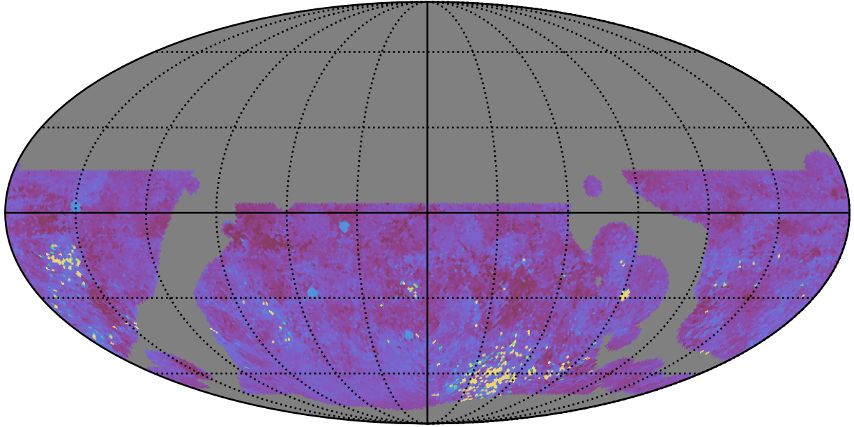
weather_cloudso0v3.5_10yrs WFD ug bands: 75th Percentile Intranight Timespan
