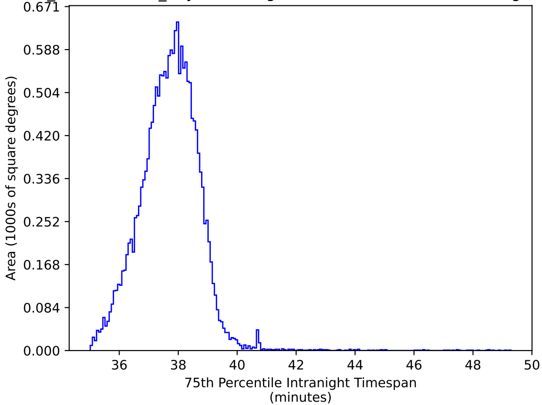
weather_cloudso0v3.5_10yrs WFD ug bands: 75th Percentile Intranight Timespan
