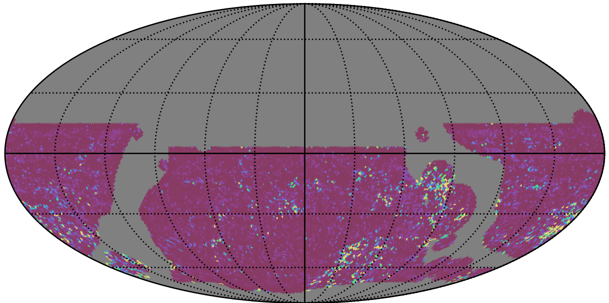
weather_cloudso0v3.5_10yrs WFD u band: 75th Percentile Intranight Timespan
