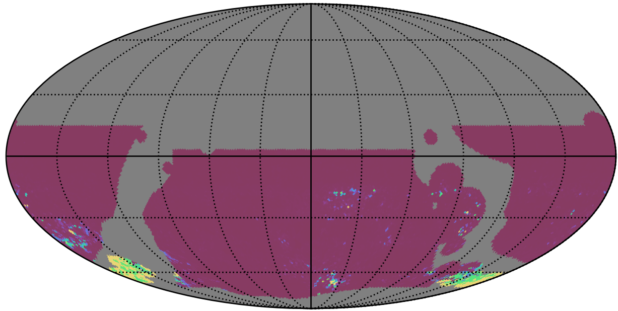
weather_cloudso0v3.5_10yrs WFD ri bands: 75th Percentile Intranight Timespan
