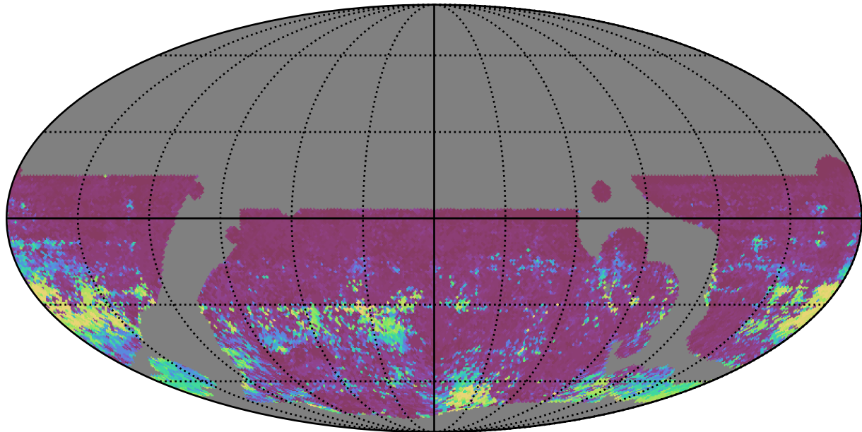
weather_cloudso0v3.5_10yrs WFD r band: 75th Percentile Intranight Timespan
