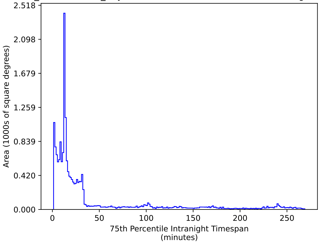
weather_cloudso0v3.5_10yrs WFD r band: 75th Percentile Intranight Timespan
