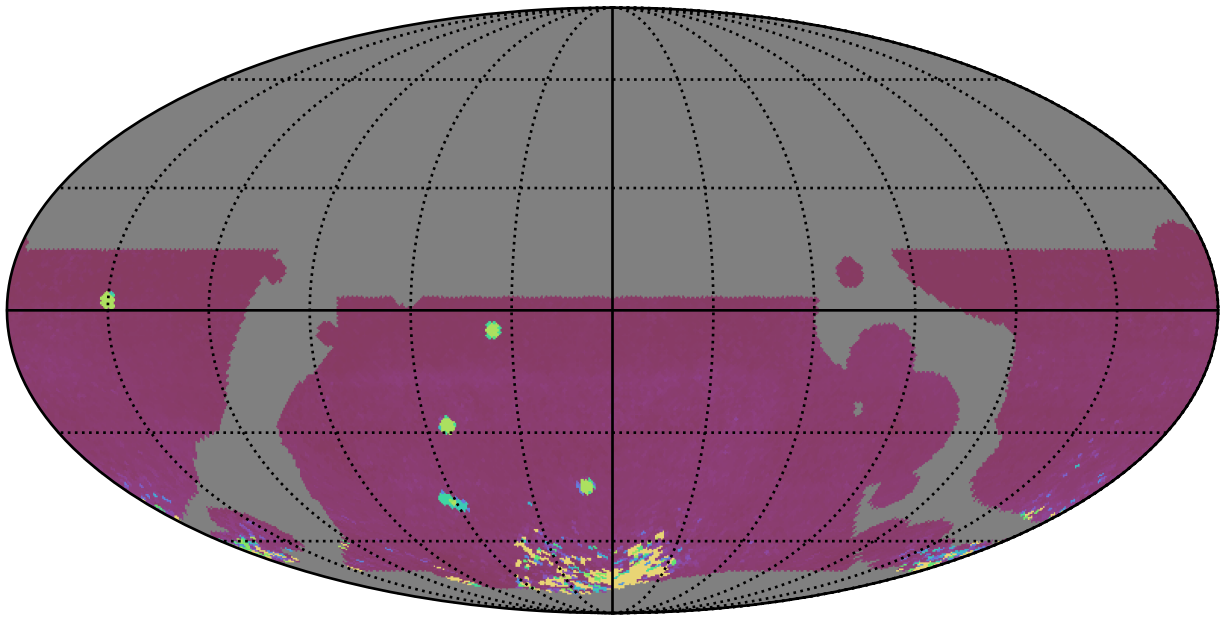
weather_cloudso0v3.5_10yrs WFD iz bands: 75th Percentile Intranight Timespan
