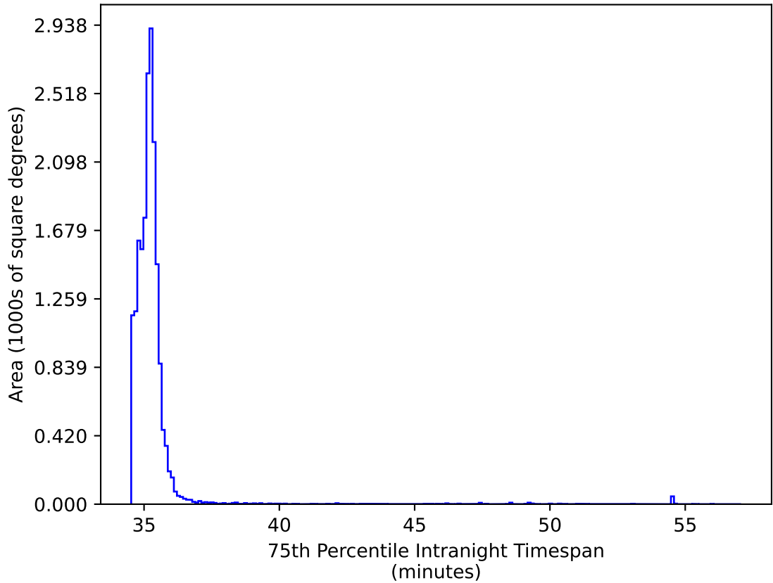
weather_cloudso0v3.5_10yrs WFD iz bands: 75th Percentile Intranight Timespan
