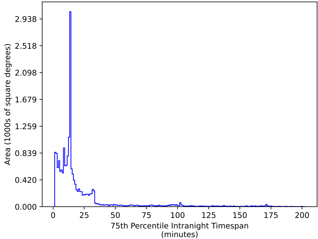
weather_cloudso0v3.5_10yrs WFD i band: 75th Percentile Intranight Timespan
