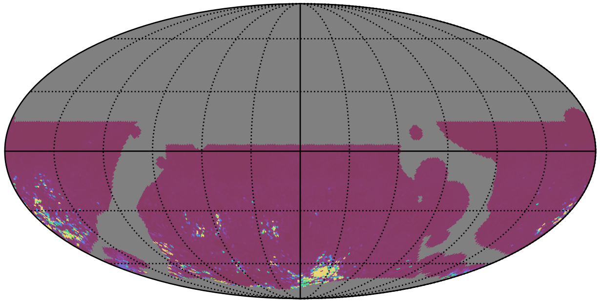
weather_cloudso0v3.5_10yrs WFD gr bands: 75th Percentile Intranight Timespan
