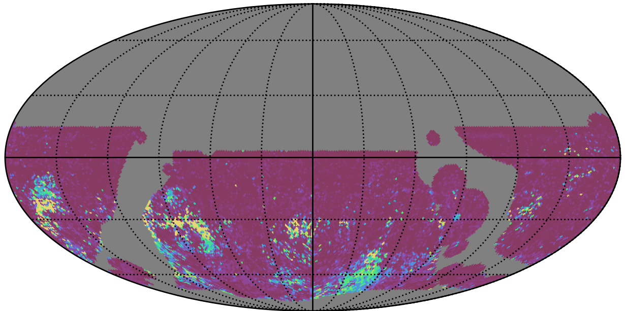
weather_cloudso0v3.5_10yrs WFD g band: 75th Percentile Intranight Timespan
