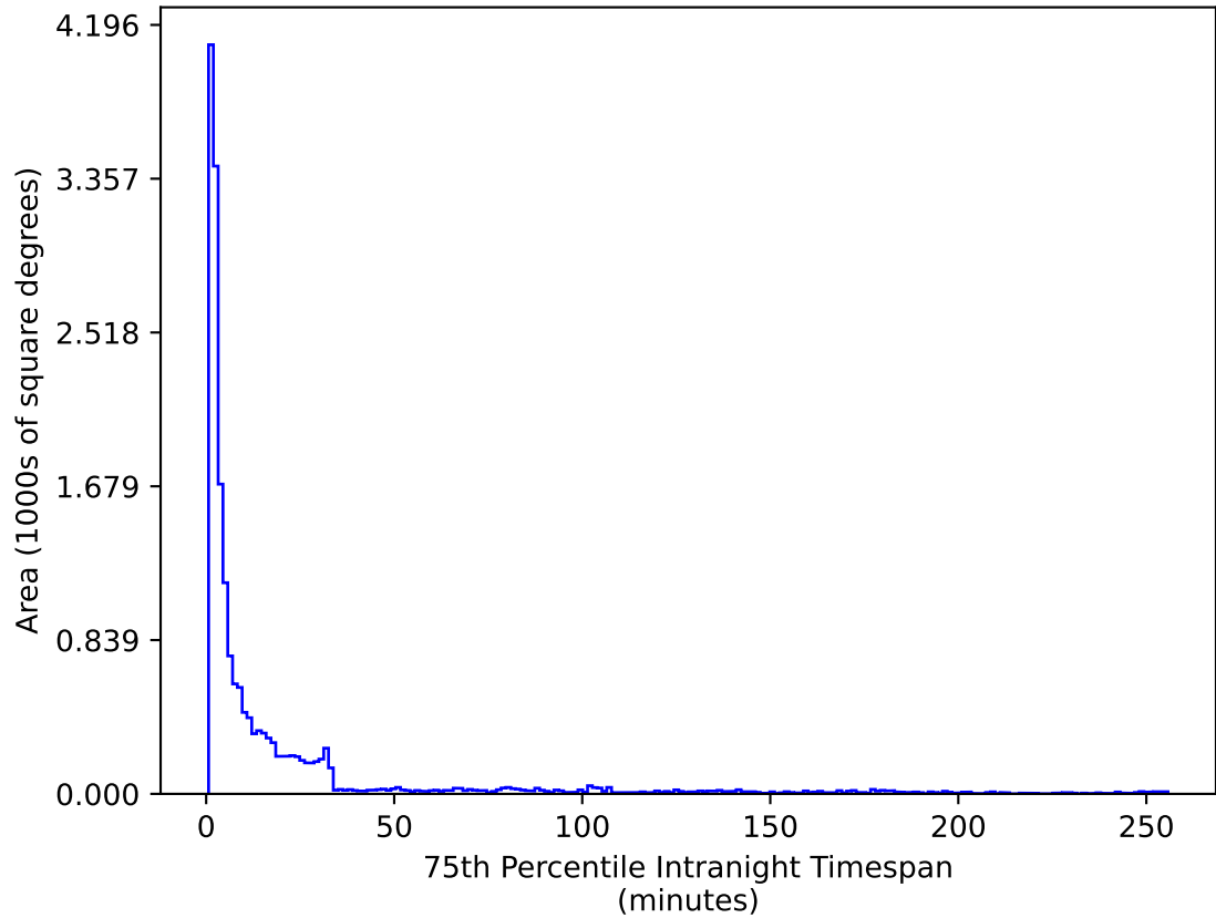
weather_cloudso0v3.5_10yrs WFD g band: 75th Percentile Intranight Timespan
