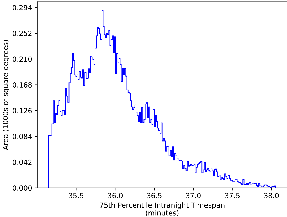
weather_cloudso0v3.5_10yrs WFD: 75th Percentile Intranight Timespan
