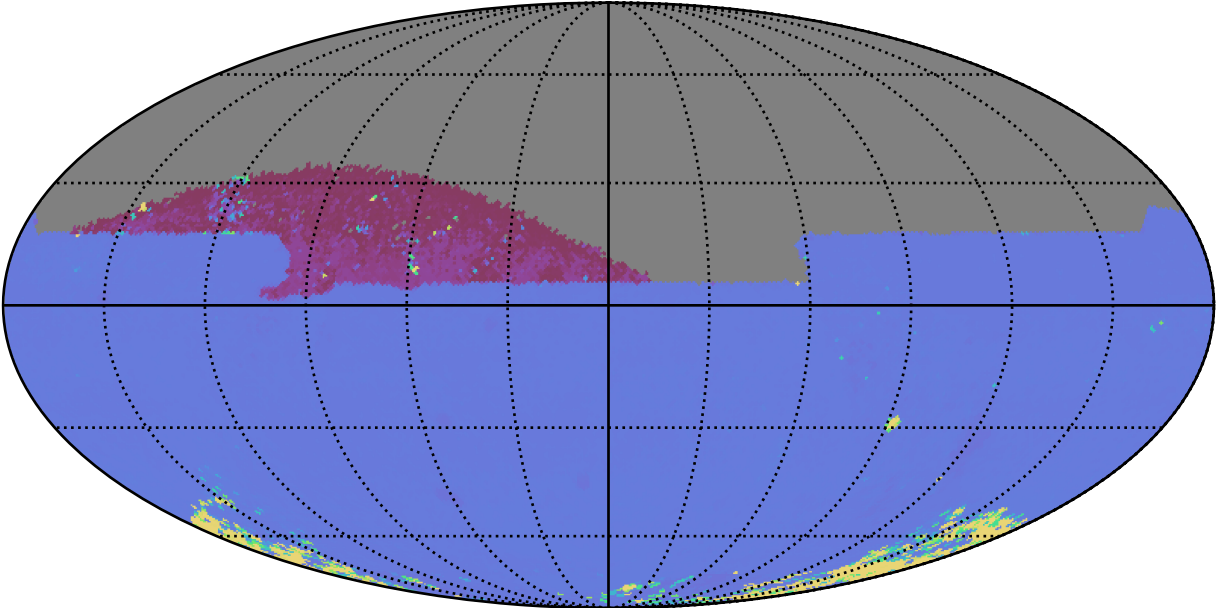
weather_cloudso0v3.5_10yrs All sky zy bands: 75th Percentile Intranight Timespan
