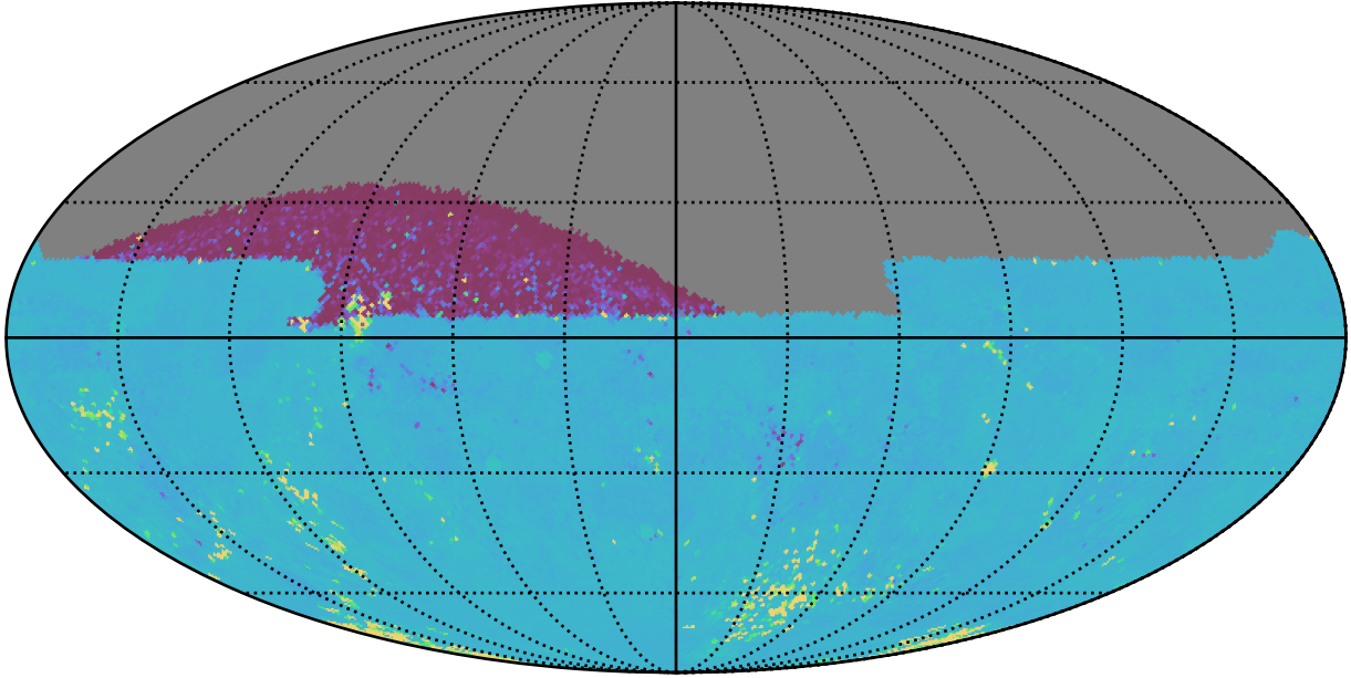
weather_cloudso0v3.5_10yrs All sky ug bands: 75th Percentile Intranight Timespan
