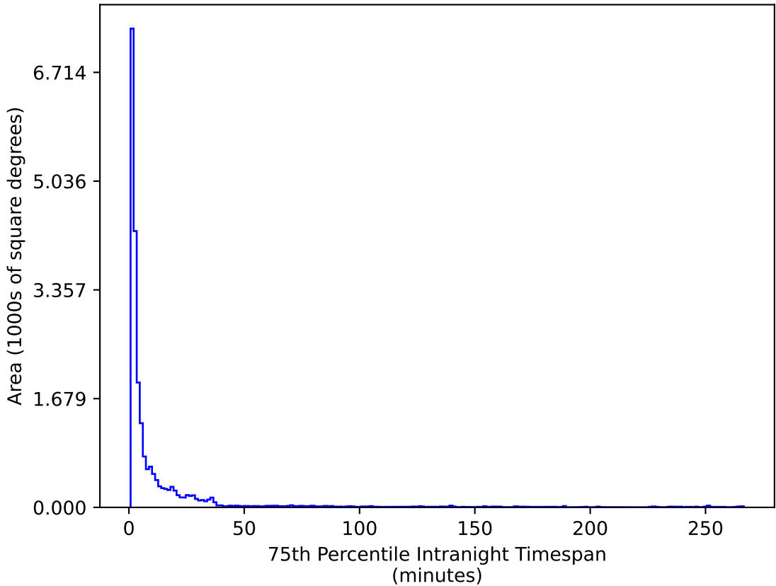
weather_cloudso0v3.5_10yrs All sky u band: 75th Percentile Intranight Timespan
