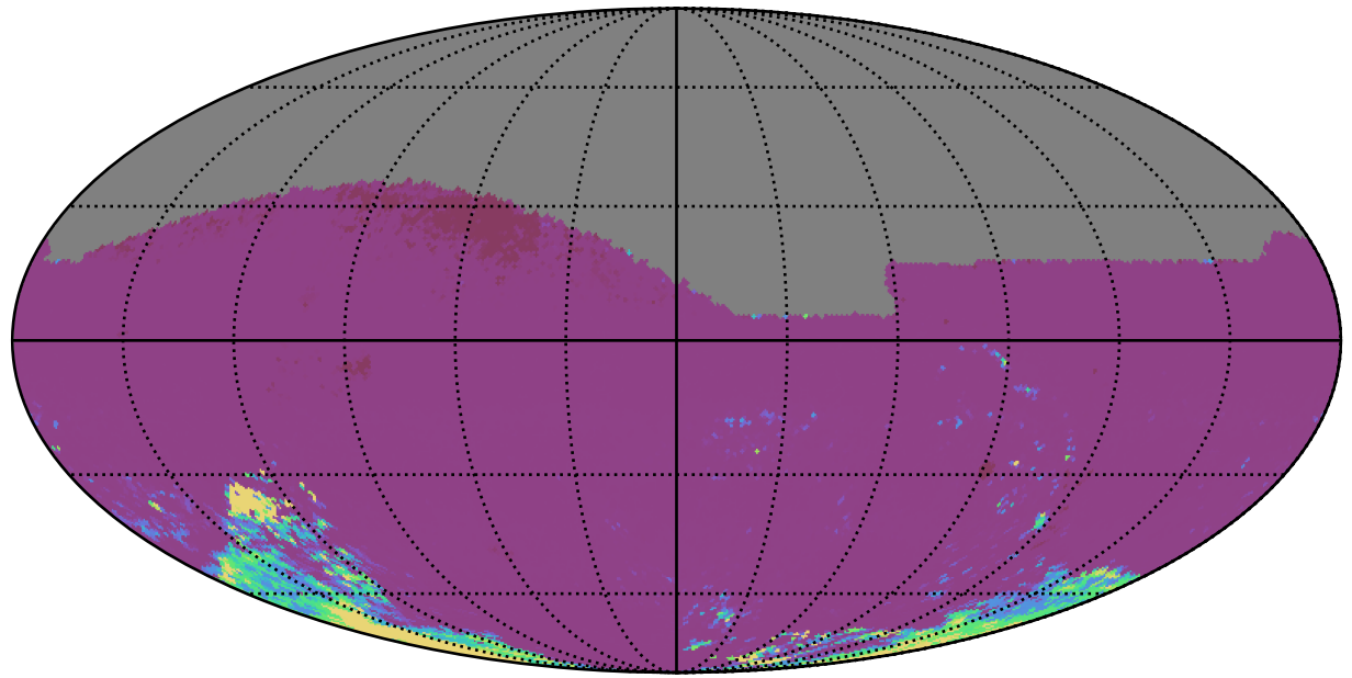
weather_cloudso0v3.5_10yrs All sky ri bands: 75th Percentile Intranight Timespan
