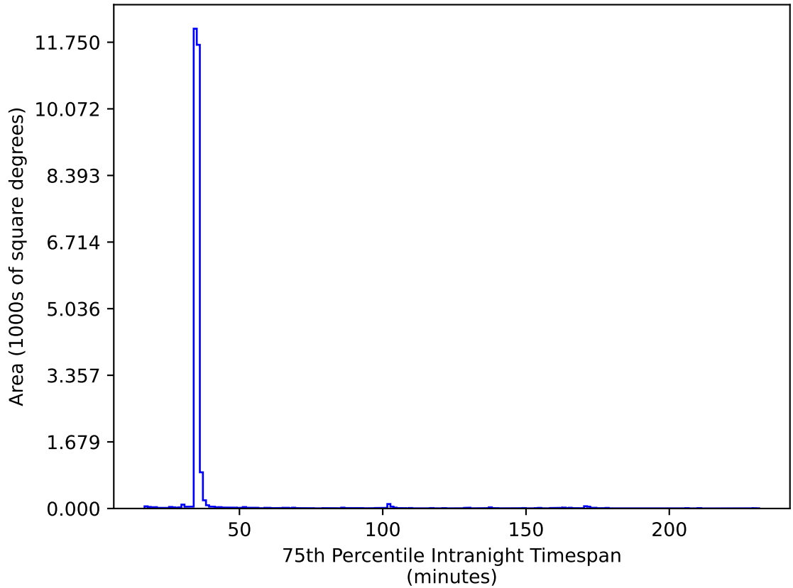
weather_cloudso0v3.5_10yrs All sky ri bands: 75th Percentile Intranight Timespan
