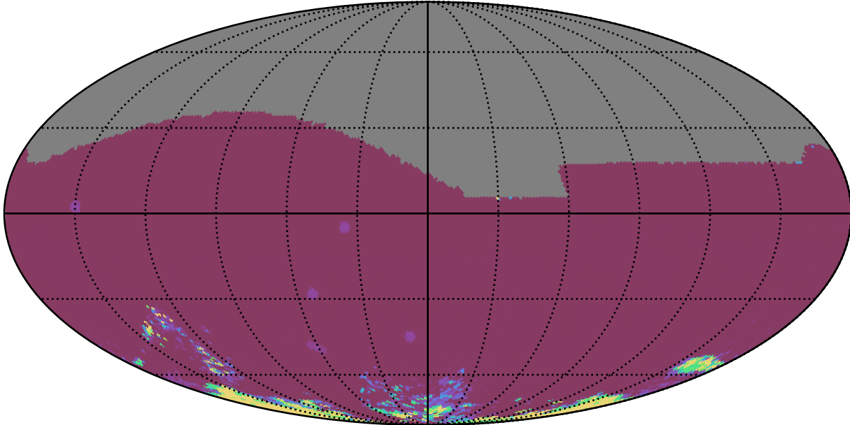
weather_cloudso0v3.5_10yrs All sky iz bands: 75th Percentile Intranight Timespan
